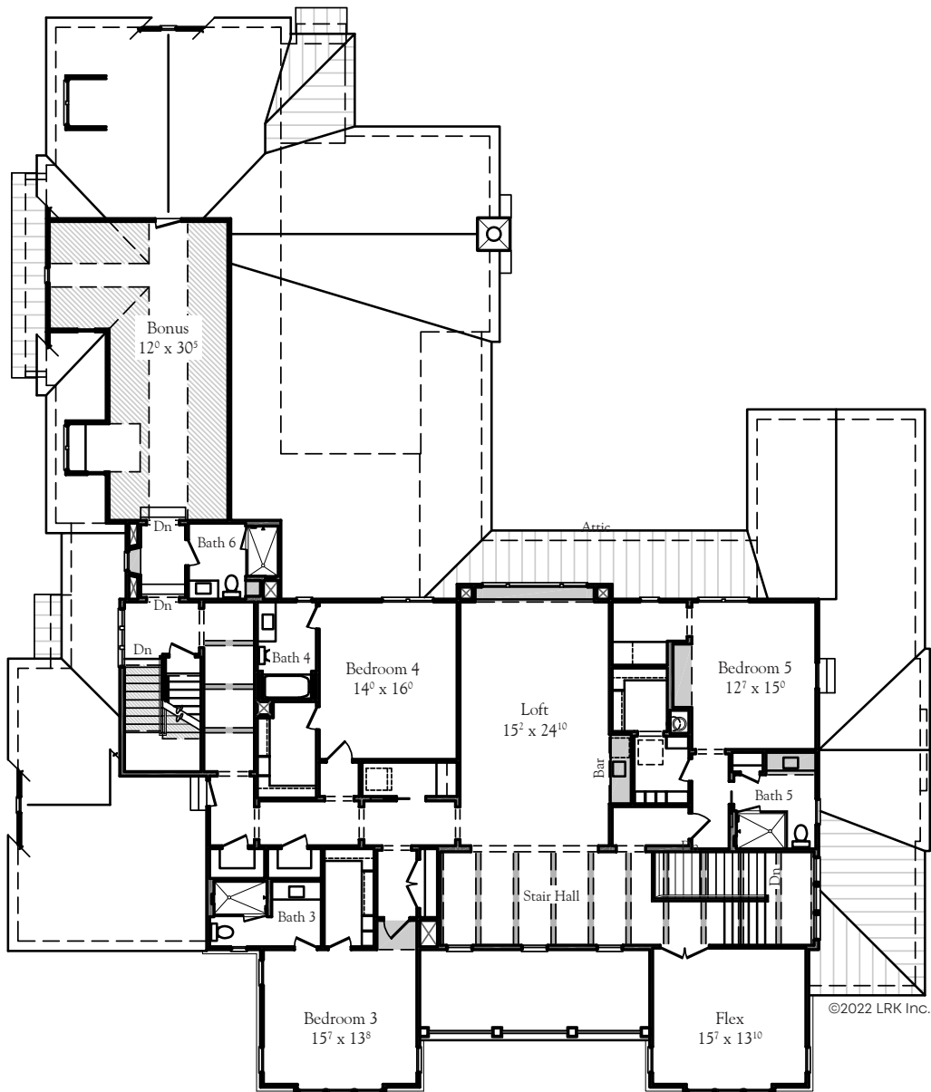
Second Floor Plan - 3,279 Sq. Ft.
